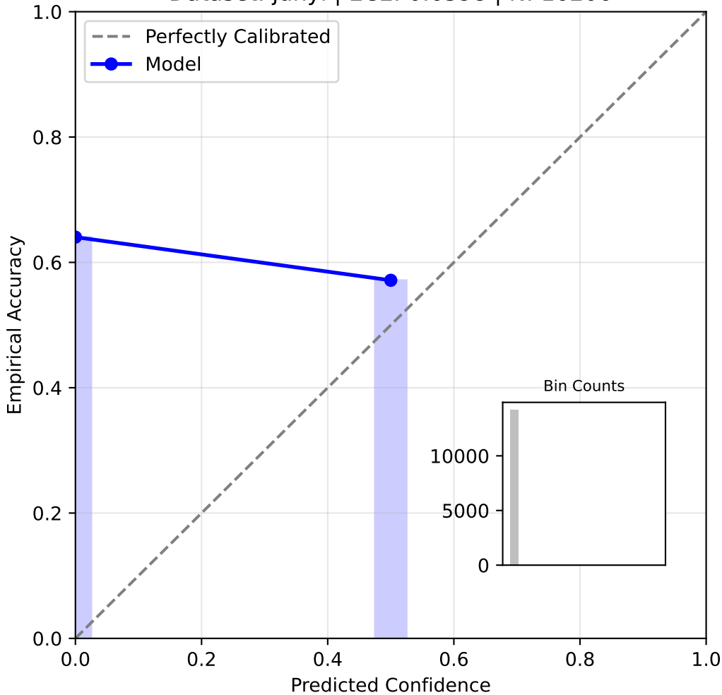
Reliability Diagram: bkt (sparse) Dataset: junyi | ECE: 0.6398 | N: 16206
