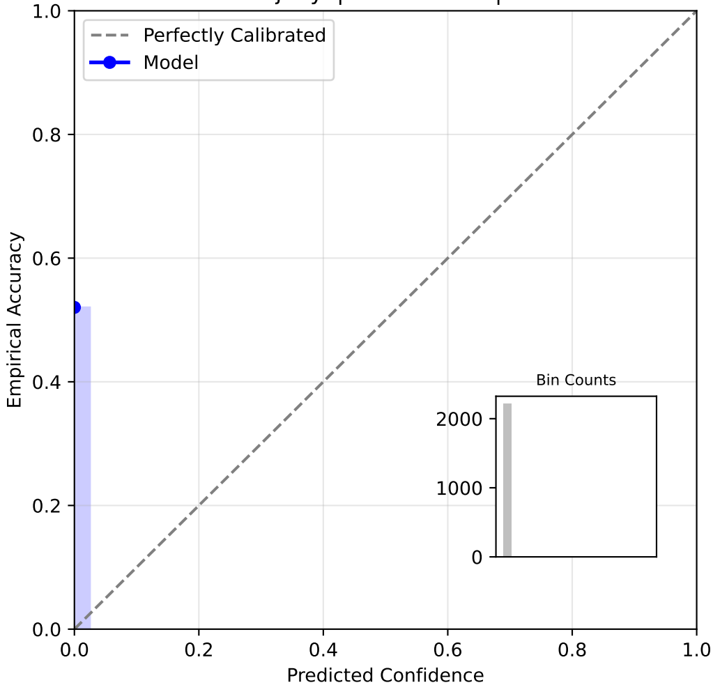
Reliability Diagram: bkt (very_sparse) Dataset: junyi | ECE: 0.5203 | N: 2545
