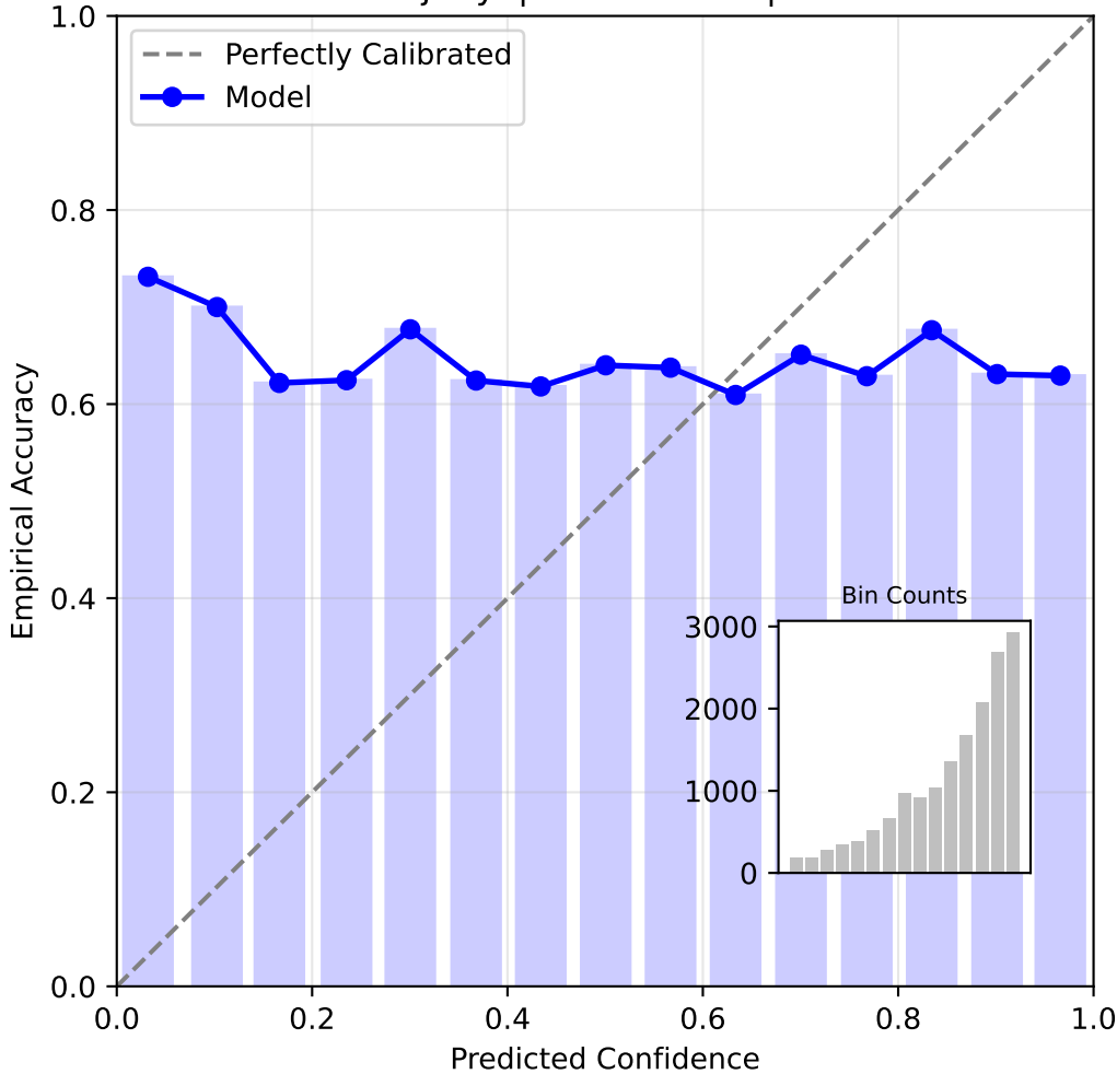
Reliability Diagram: dkt (sparse) Dataset: junyi | ECE: 0.2139 | N: 16206
