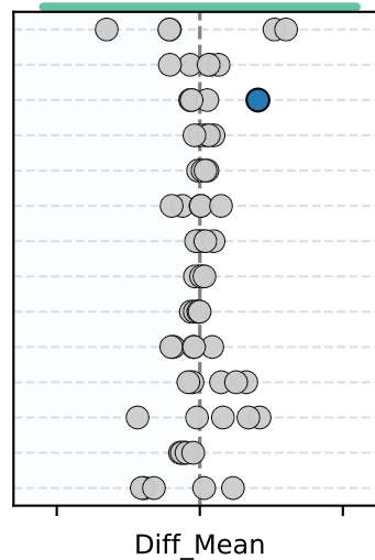
Gaussian Copula
