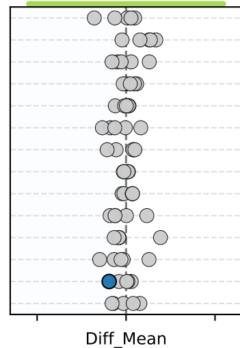
Synthpop
