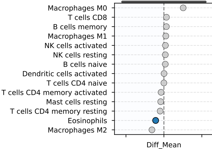
CTGAN
