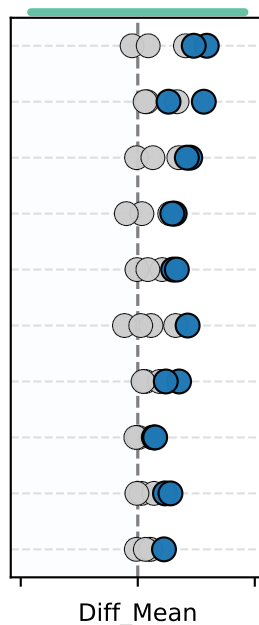
Synthpop
