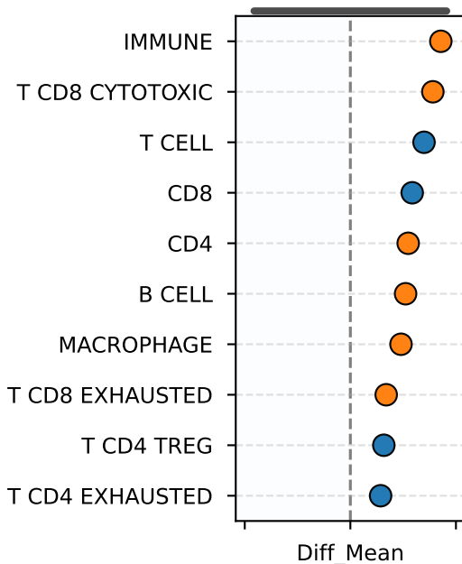
Gaussian Copula
