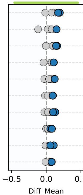
Synthpop
