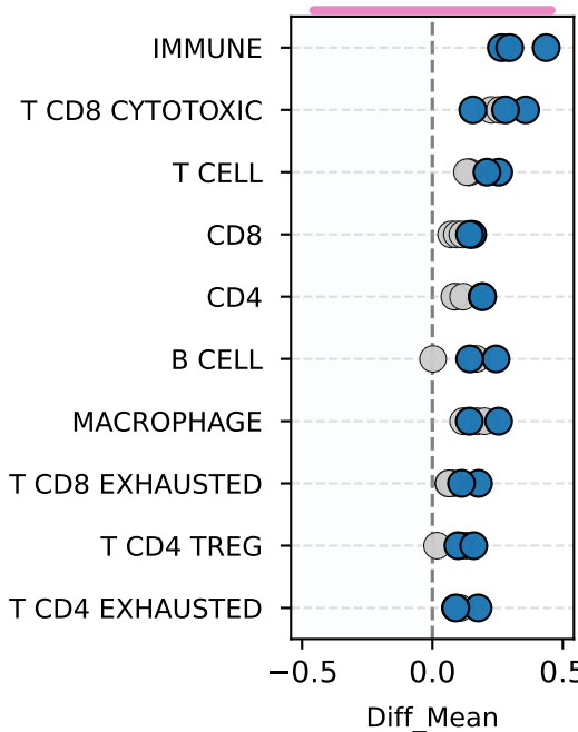
Gaussian Copula
