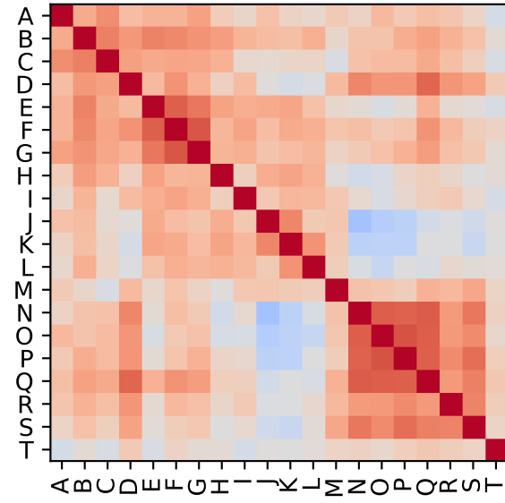
Gaussian Copula
