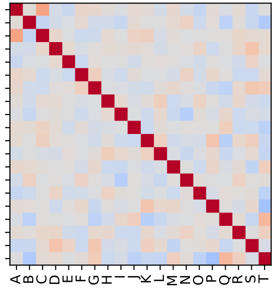
CTGAN
