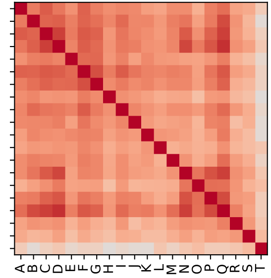
Synthpop
