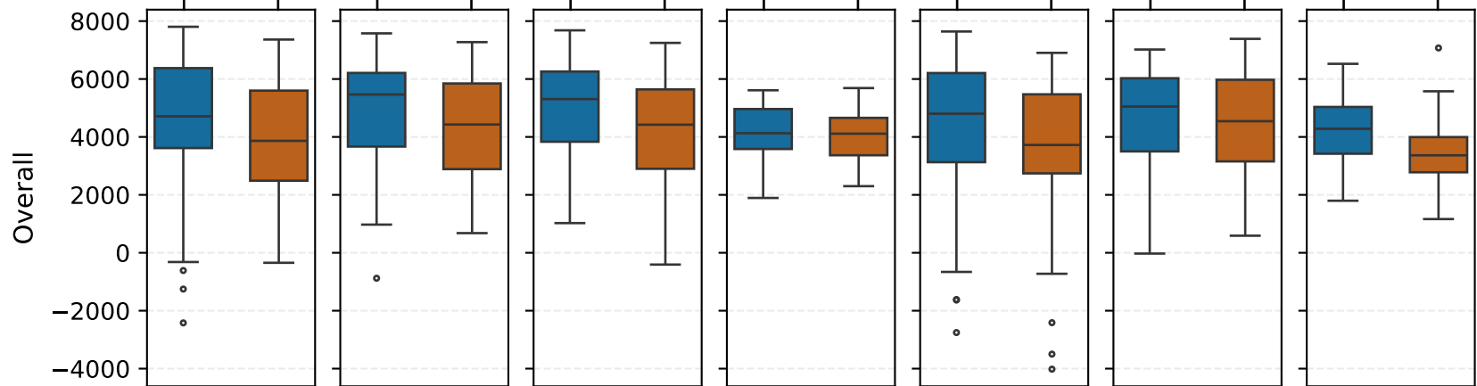
Original Data Avatars K5 Avatars K10 CTGAN Gaussian Copula Synthpop TVAE ** (p=0.0322) * (p=0.051) ** (p=0.0388) NS (p=0.403) NS (p=0.163) NS (p=0.563) *** (p=0.00197)
