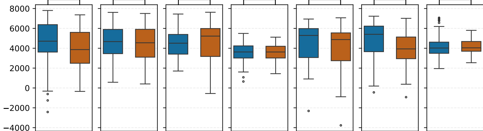
Original Data Avatars K5 Avatars K10 CTGAN Gaussian Copula Synthpop TVAE ** (p=0.0322) NS (p=0.905) NS (p=0.272) NS (p=0.948) NS (p=0.142) ** (p=0.0215) NS (p=0.781)
