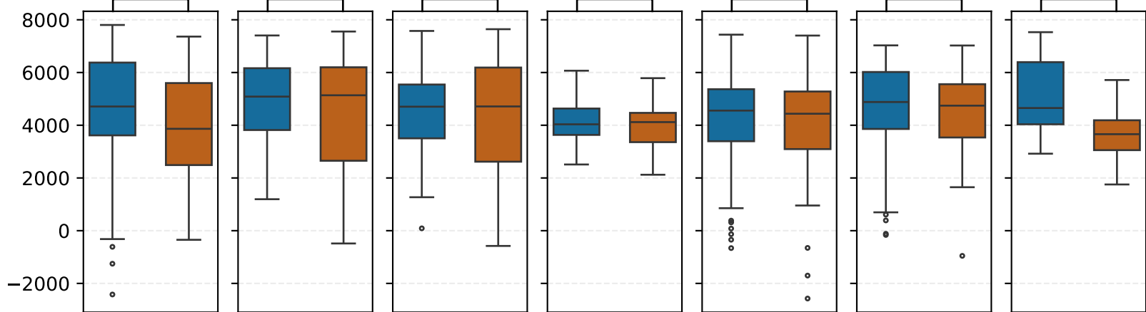
Original Data Avatars K5 Avatars K10 CTGAN Gaussian Copula Synthpop TVAE ** (p=0.0322) NS (p=0.366) NS (p=0.932) NS (p=0.403) NS (p=0.6) NS (p=0.345) *** (p=8.44e-09)
