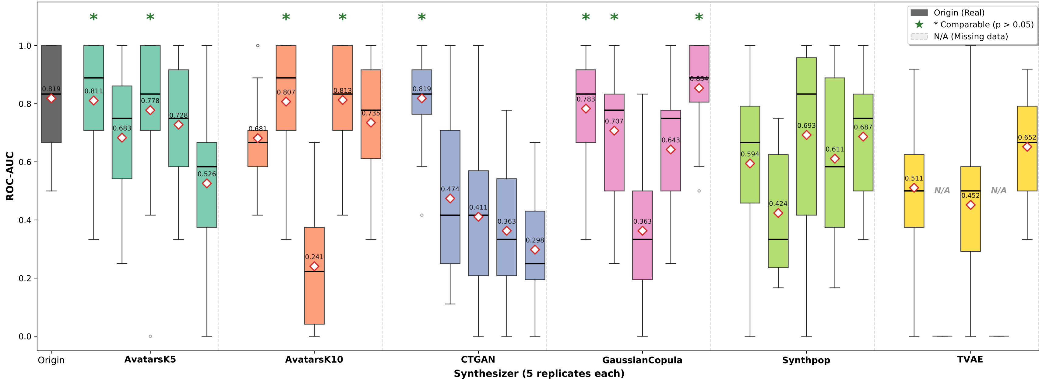
ROC-AUC Distribution: Logistic Regression Across 5 Seeds
