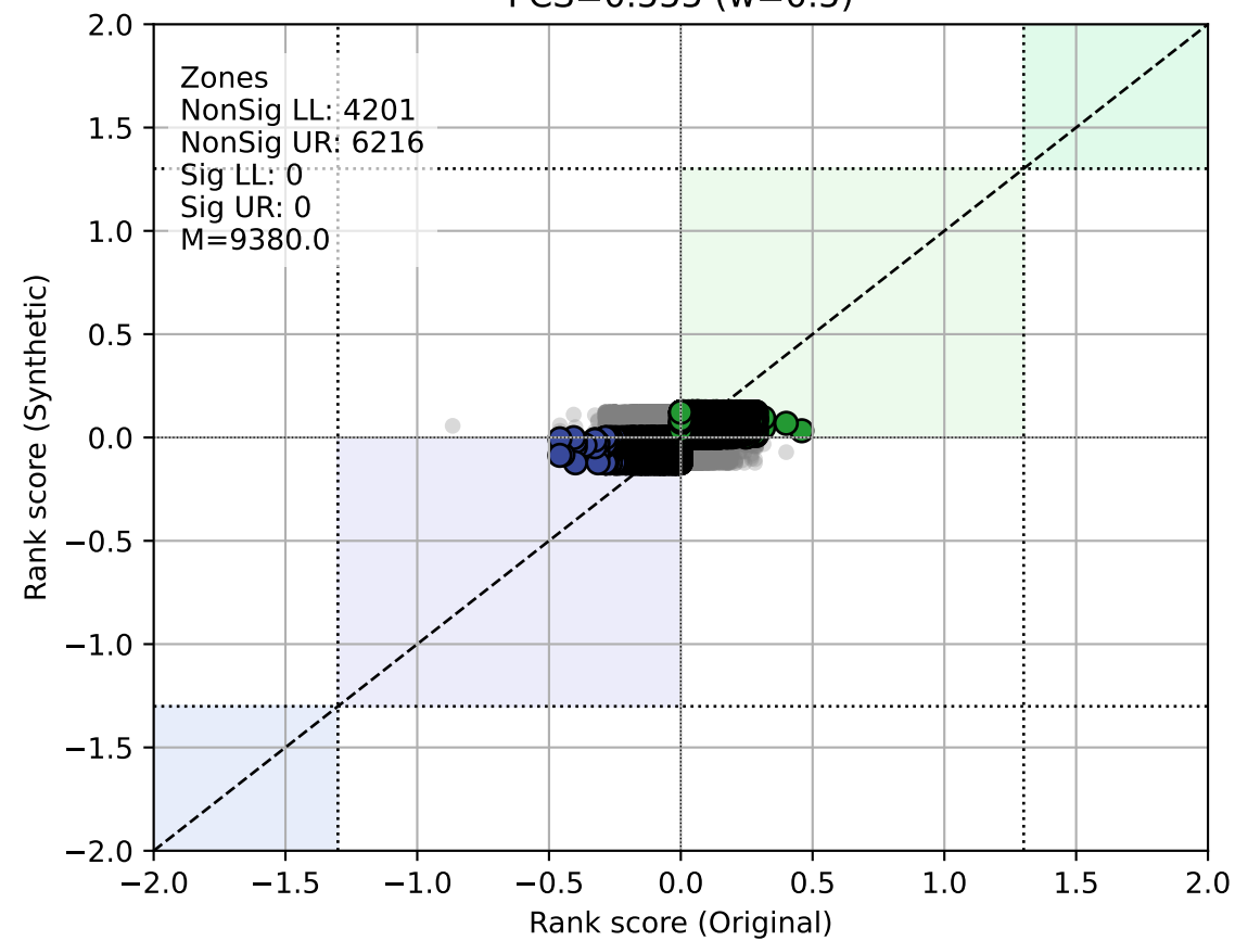
Synthpop PCS=0.555 (w=0.5)
