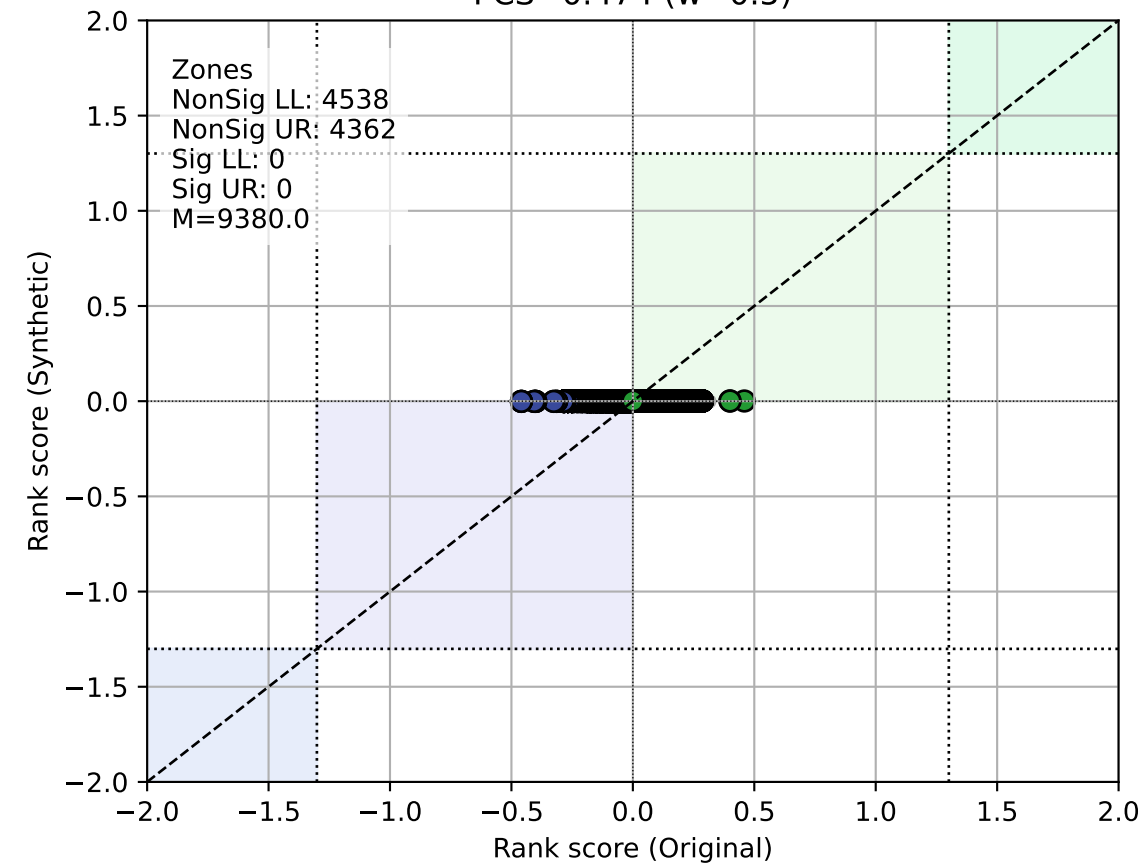
TVAE PCS=0.561 (w=0.5)
