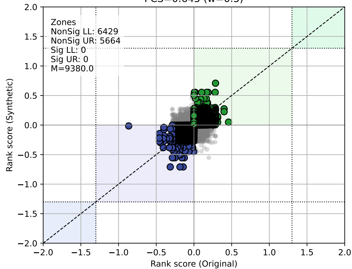
Gaussian Copula PCS=0.645 (w=0.5)
