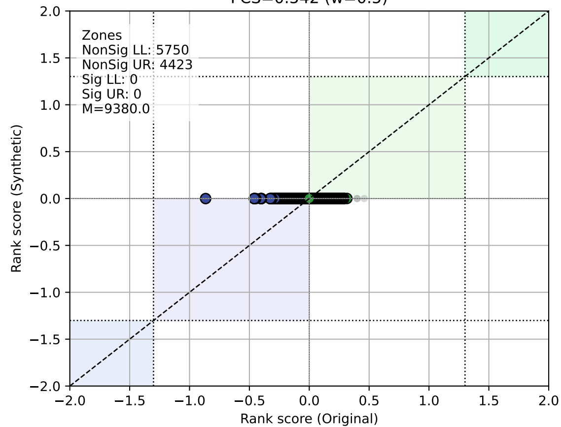
Synthpop PCS=0.542 (w=0.5)
