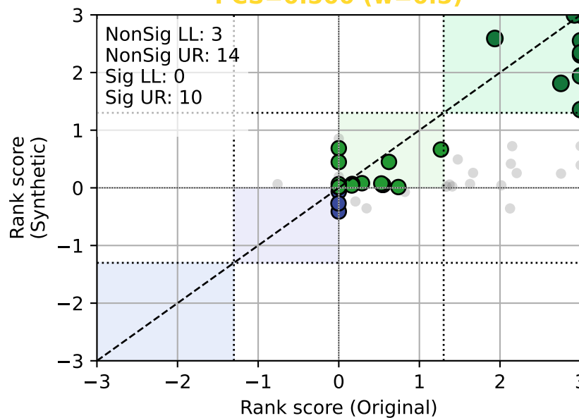
TVAE PCS=0.500 (w=0.5)
