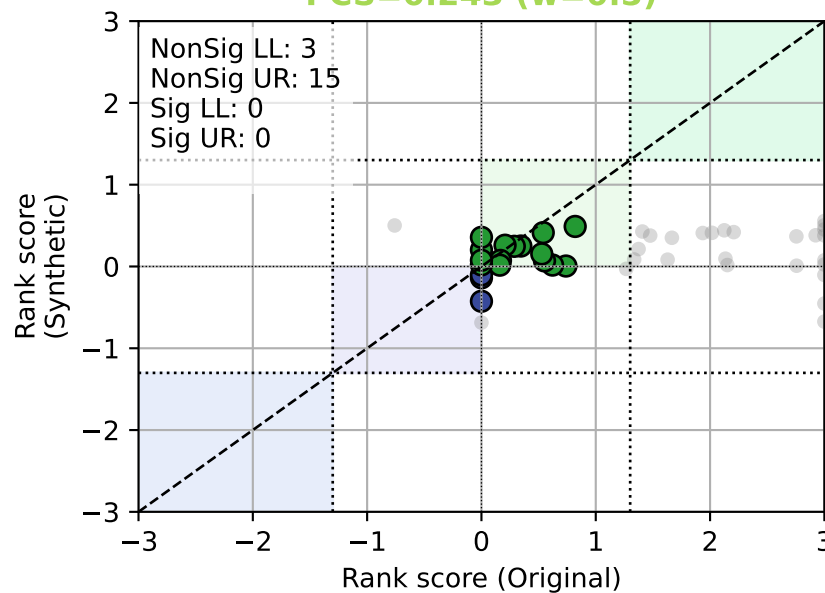
Synthpop PCS=0.243 (w=0.5)
