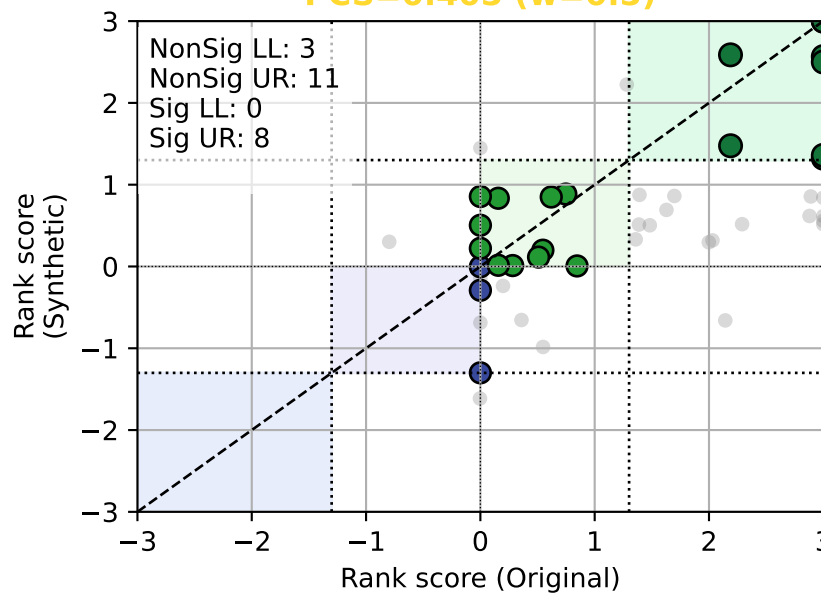
TVAE PCS=0.405 (w=0.5)
