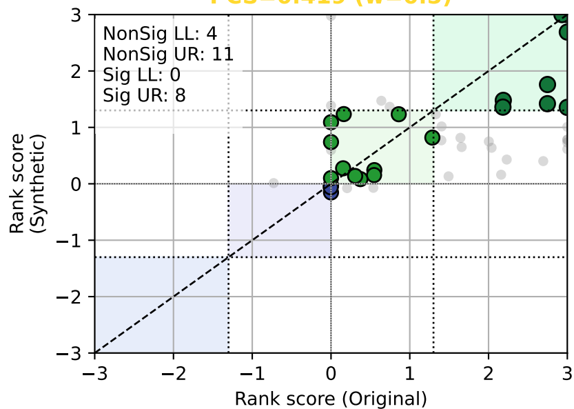
TVAE PCS=0.419 (w=0.5)
