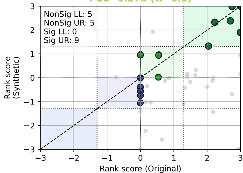
Synthpop PCS=0.378 (w=0.5)
