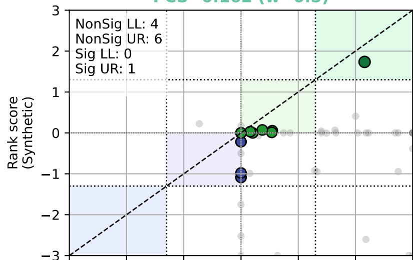
CTGAN PCS=0.162 (w=0.5)
