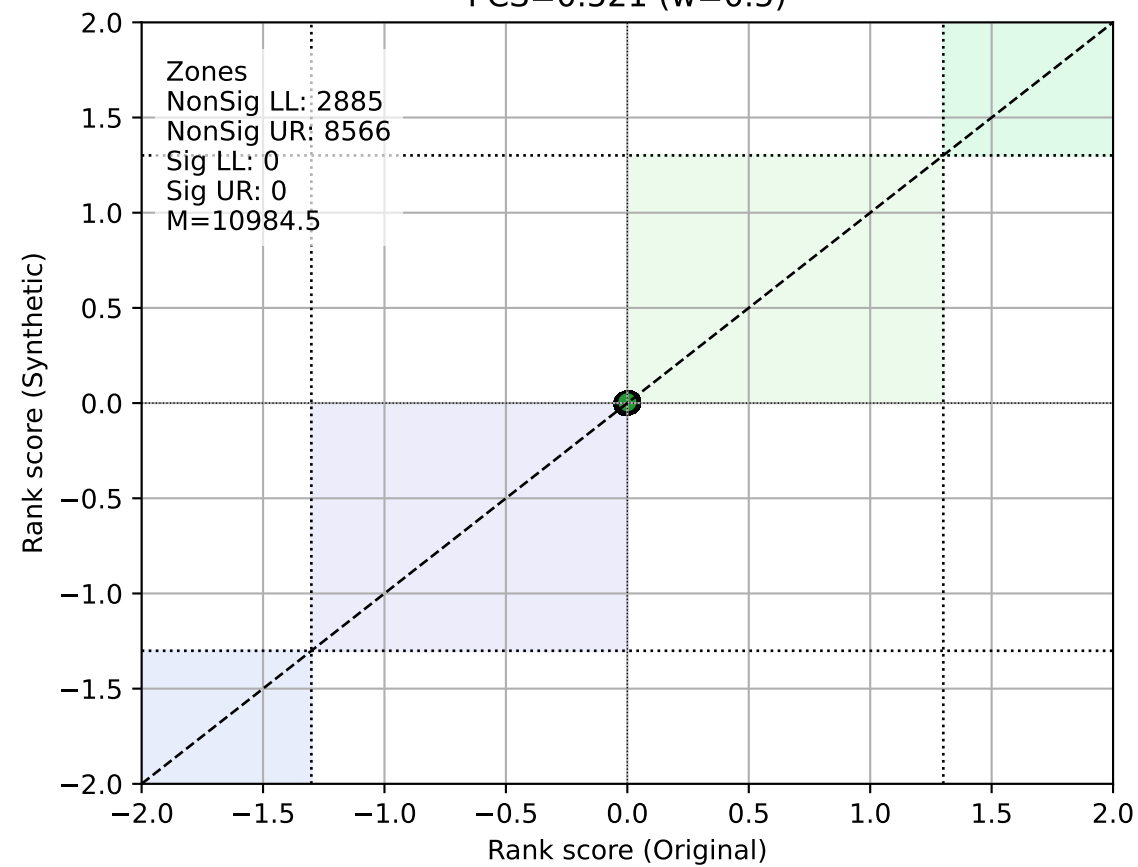
Synthpop PCS=0.521 (w=0.5)
