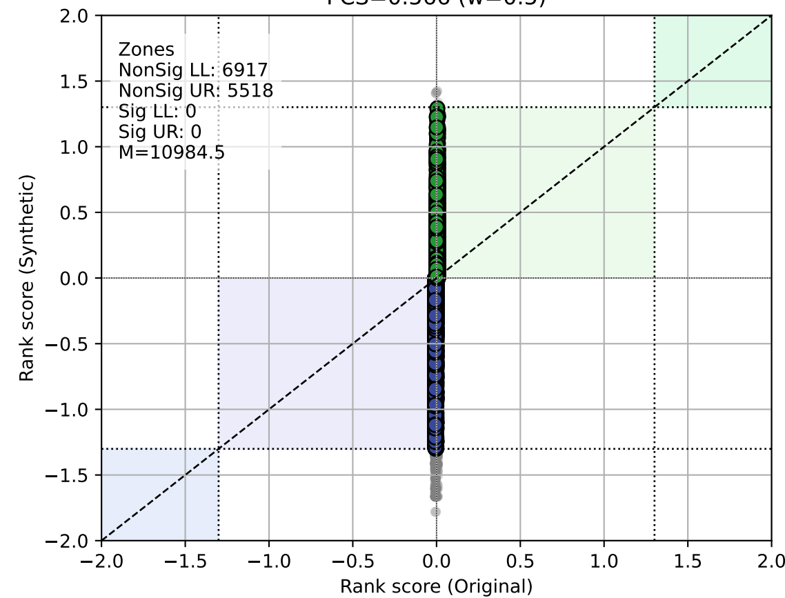
TVAE PCS=0.566 (w=0.5)
