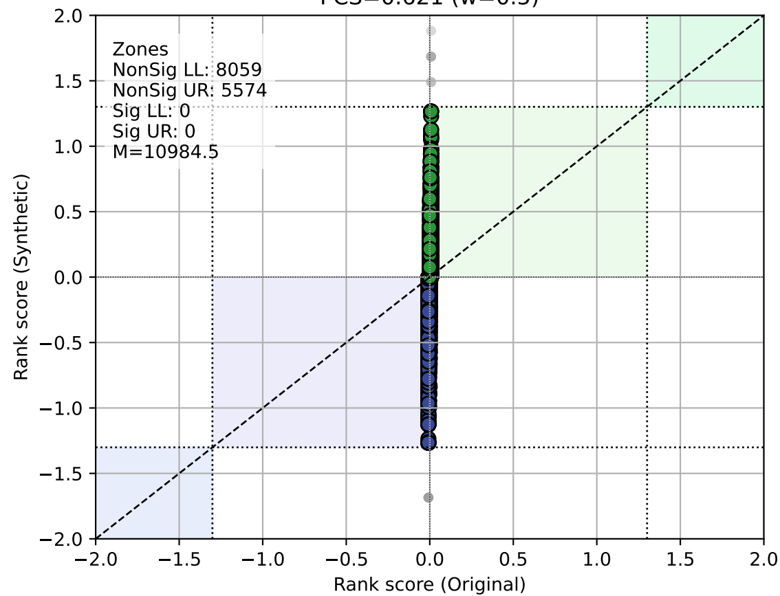
Gaussian Copula PCS=0.621 (w=0.5)
