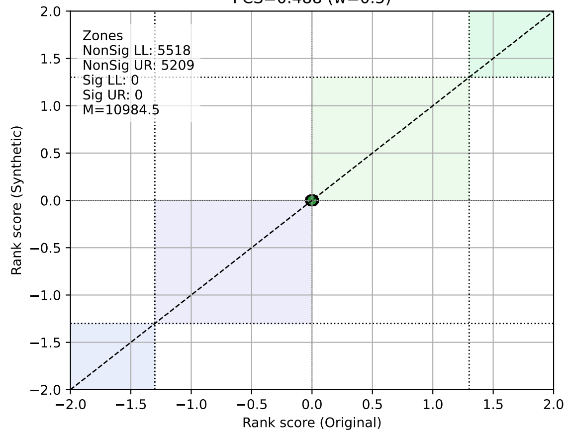
Synthpop PCS=0.488 (w=0.5)
