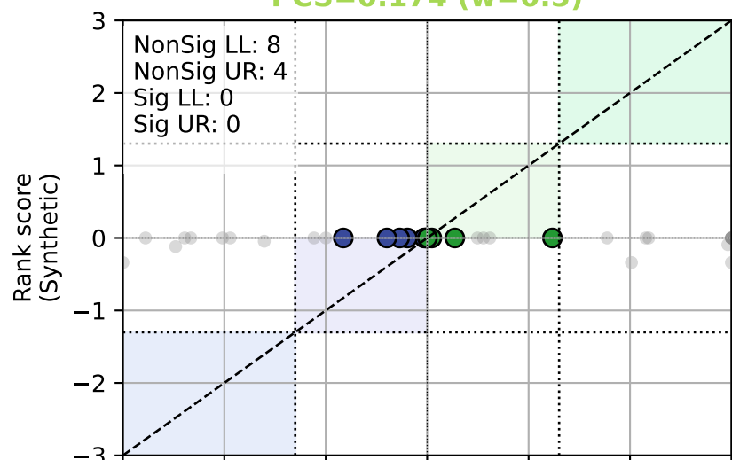
Synthpop PCS=0.174 (w=0.5)
