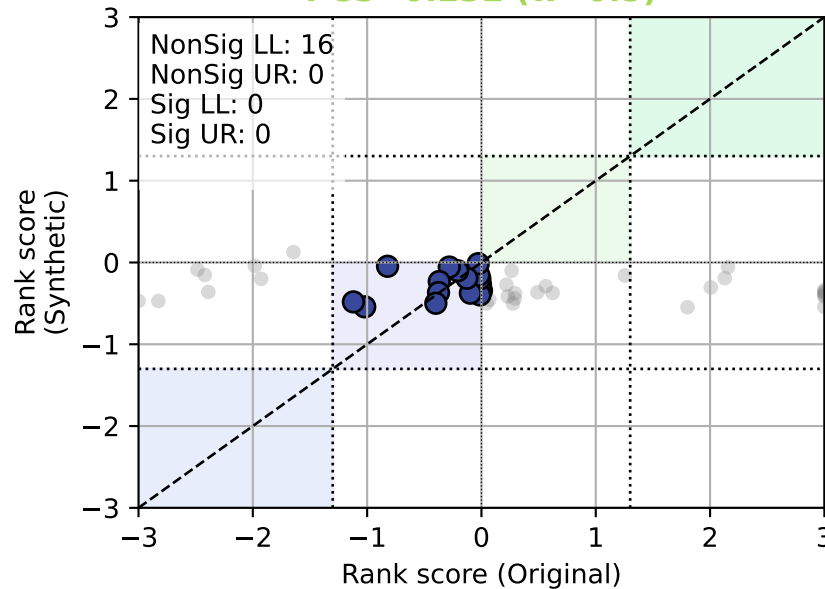
Synthpop PCS=0.232 (w=0.5)
