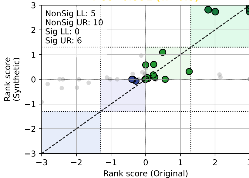
TVAE PCS=0.391 (w=0.5)
