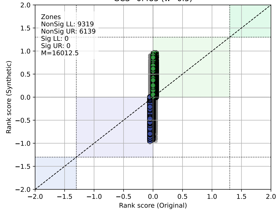
Synthpop GCS=0.483 (w=0.5)
