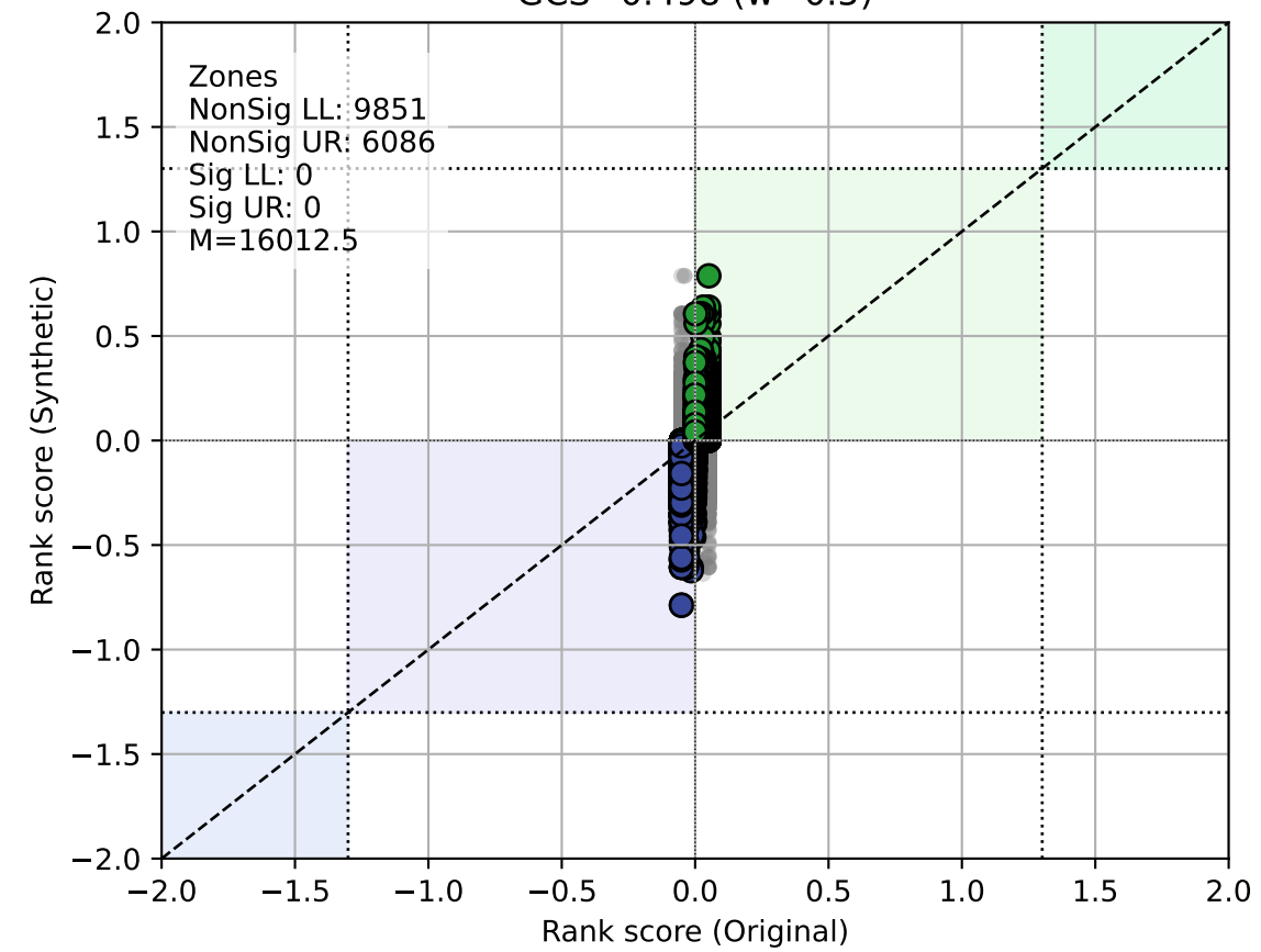
CTGAN GCS=0.498 (w=0.5)
