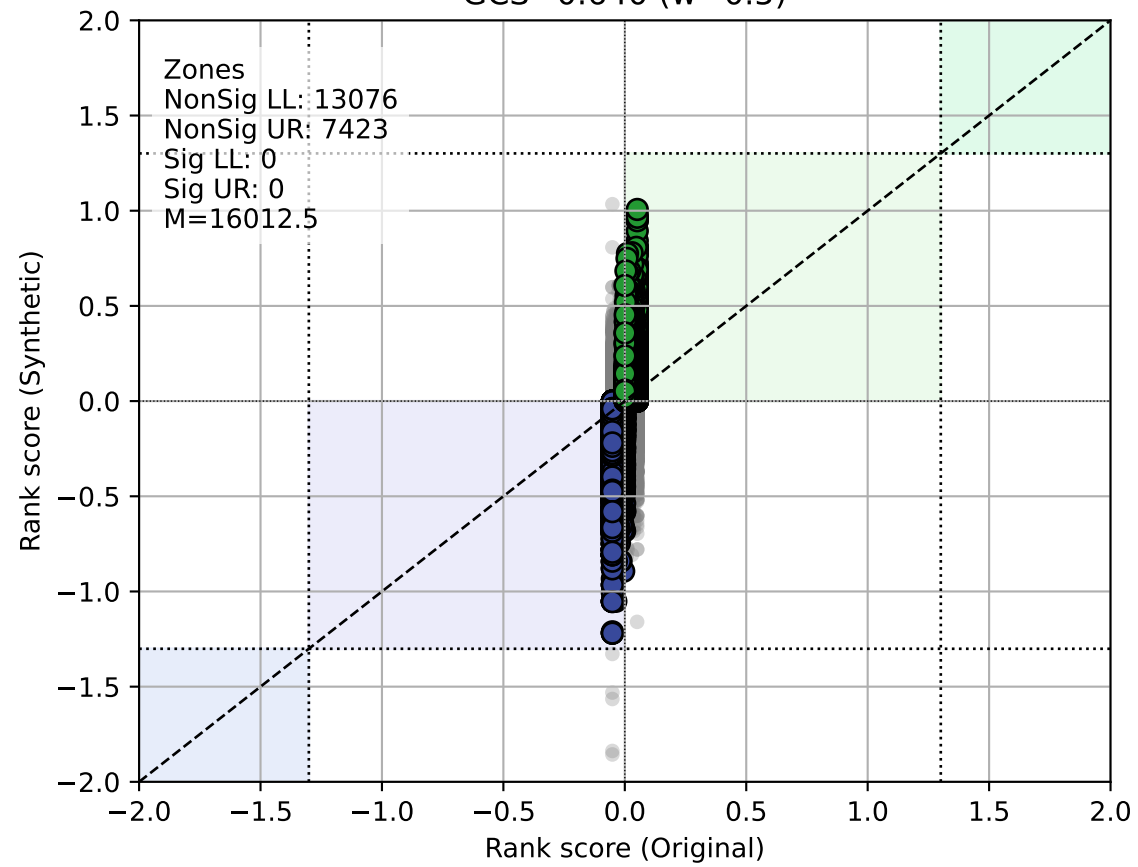
Gaussian Copula GCS=0.640 (w=0.5)
