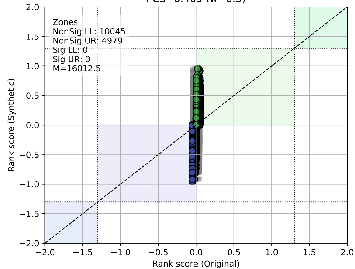
Synthpop PCS=0.469 (w=0.5)
