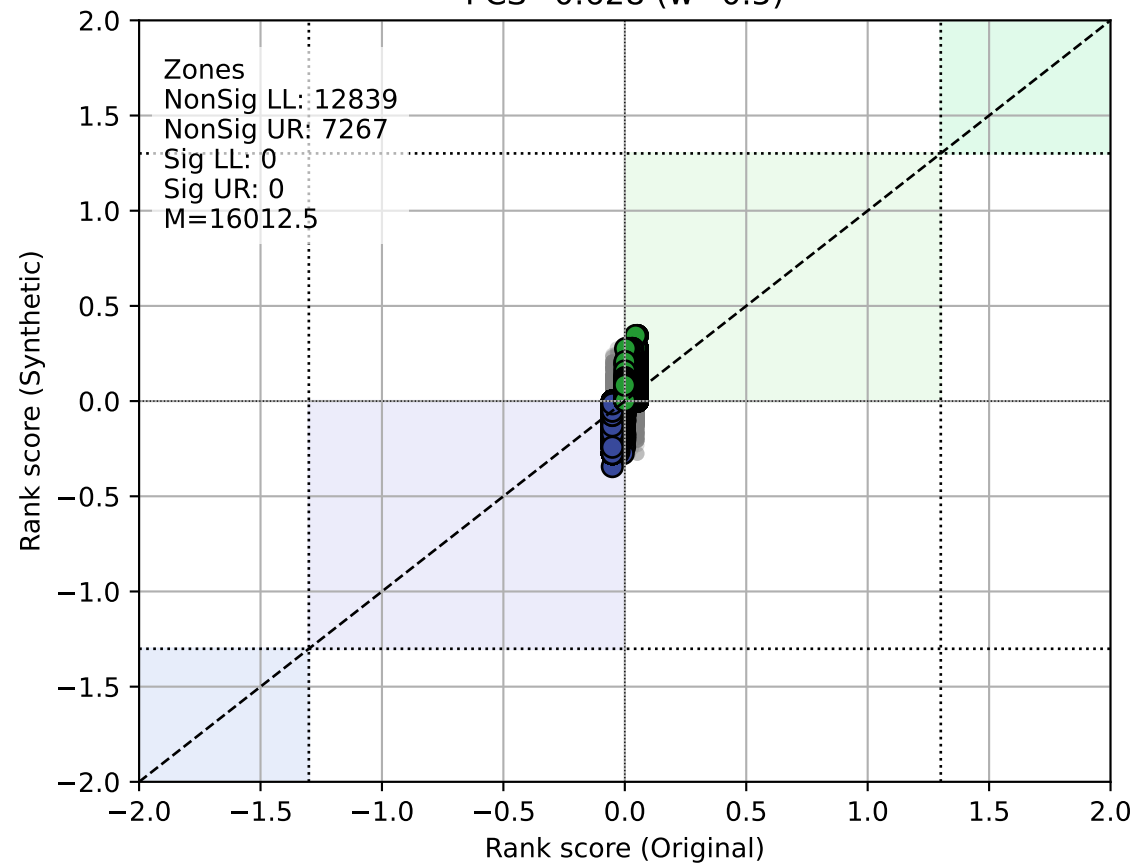
Gaussian Copula PCS=0.628 (w=0.5)
