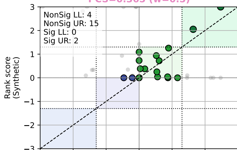
Gaussian Copula PCS=0.365 (w=0.5)
