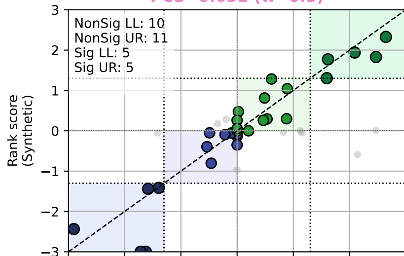
Gaussian Copula PCS=0.651 (w=0.5)
