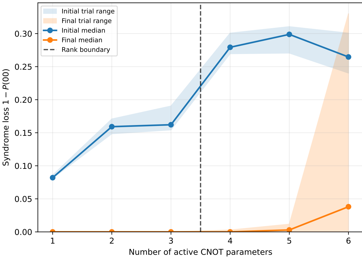
Circuit-level optimization
