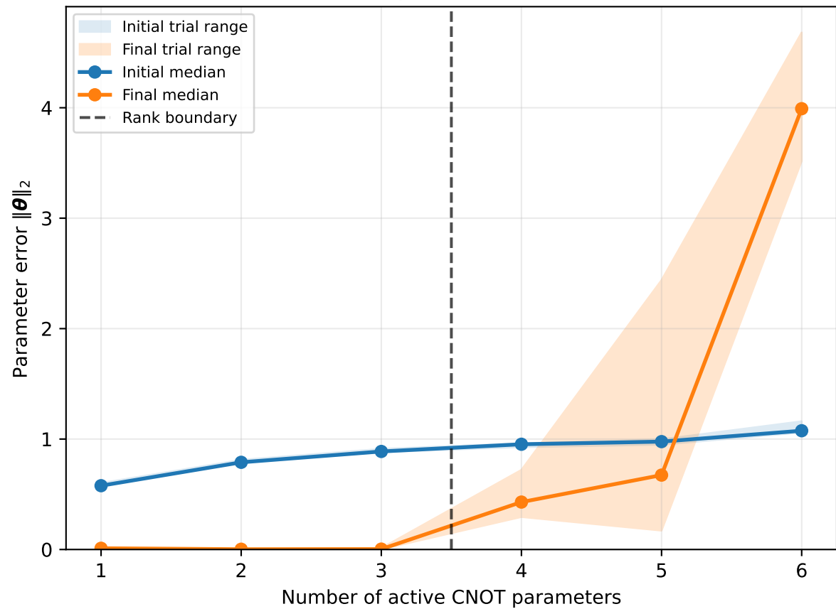
Individual-parameter recovery
