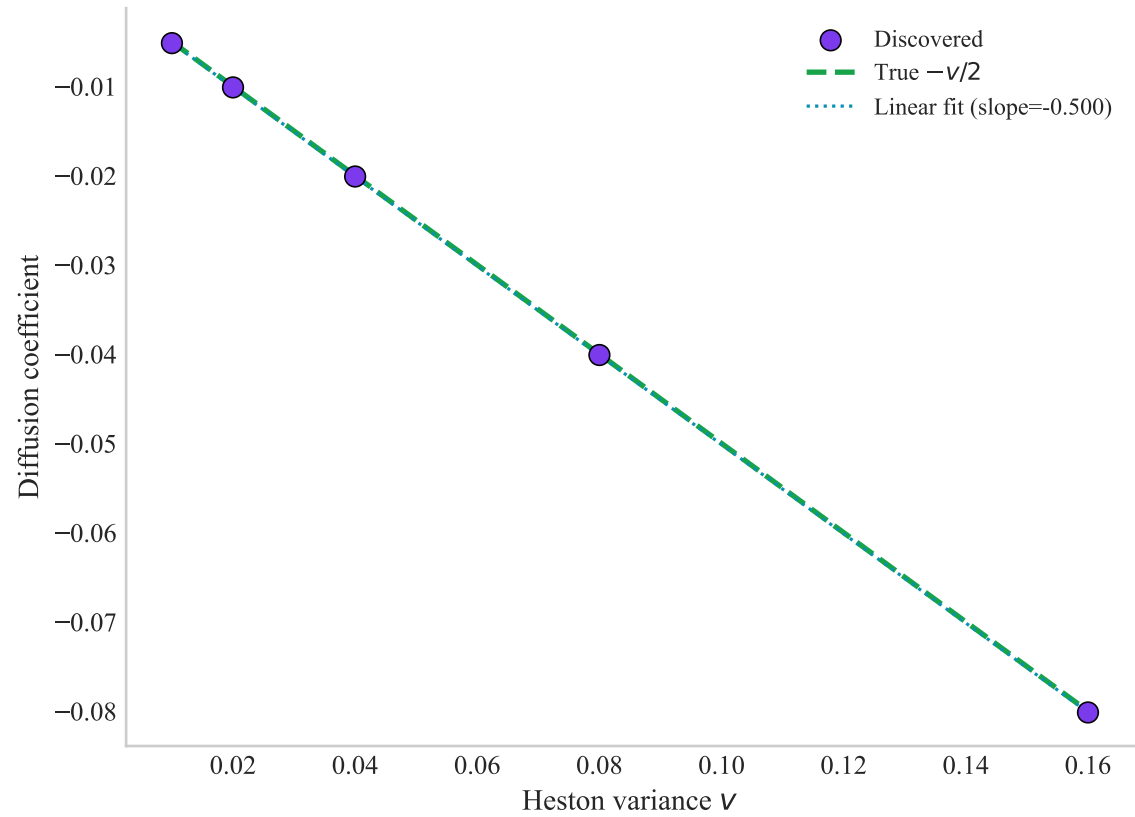
Heston: linear v scaling of \sigma^2
