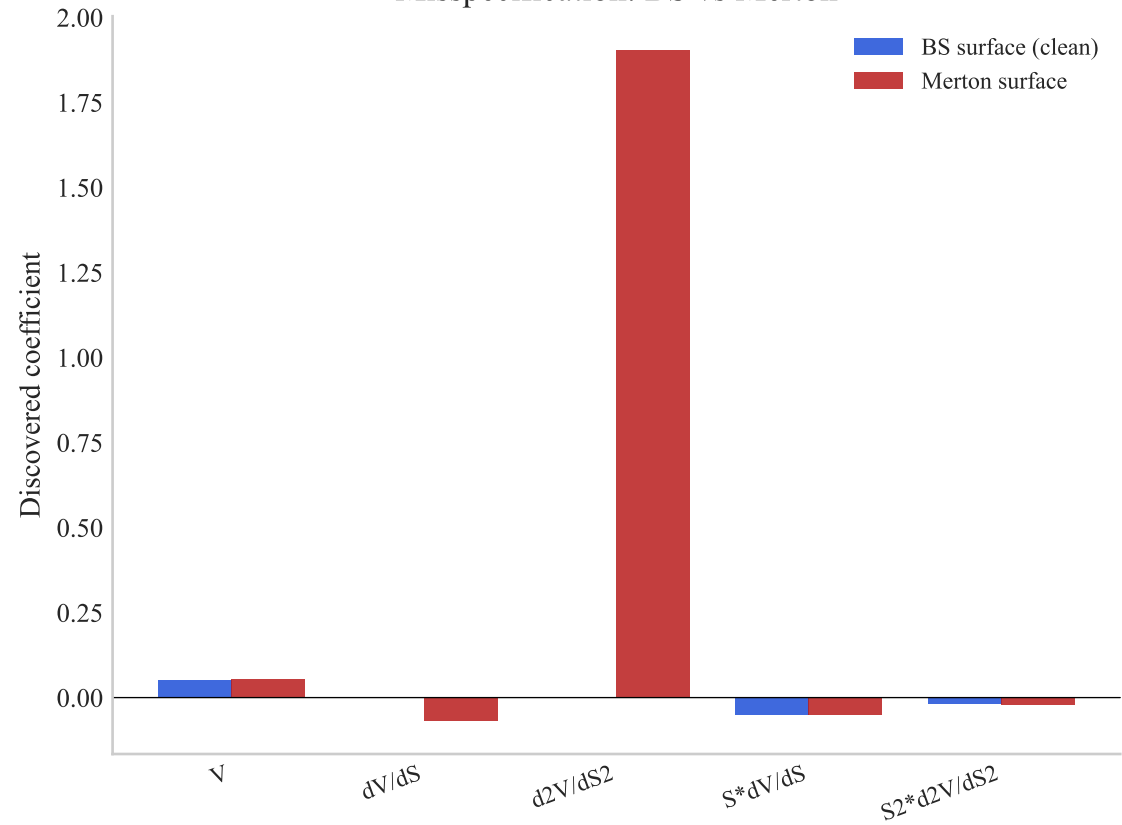
Misspecification: BS vs Merton
