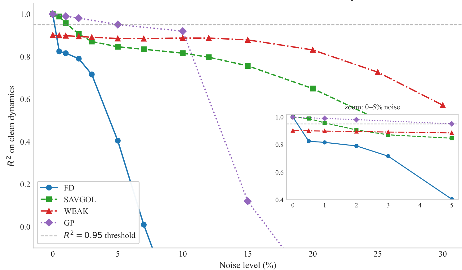
Noise robustness: derivative estimators for SINDy
