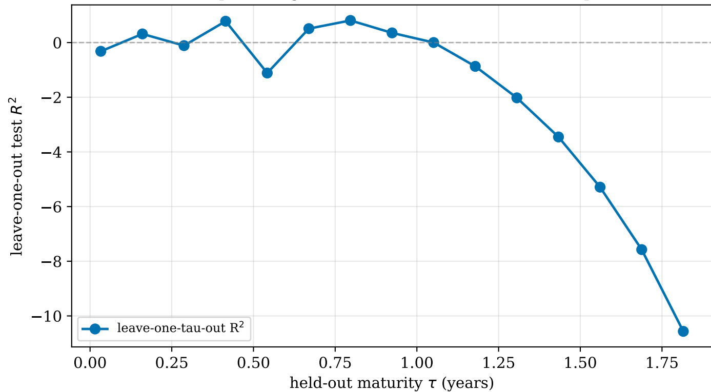
Per-expiration generalization of the [2, 1] KAN-Dupire
