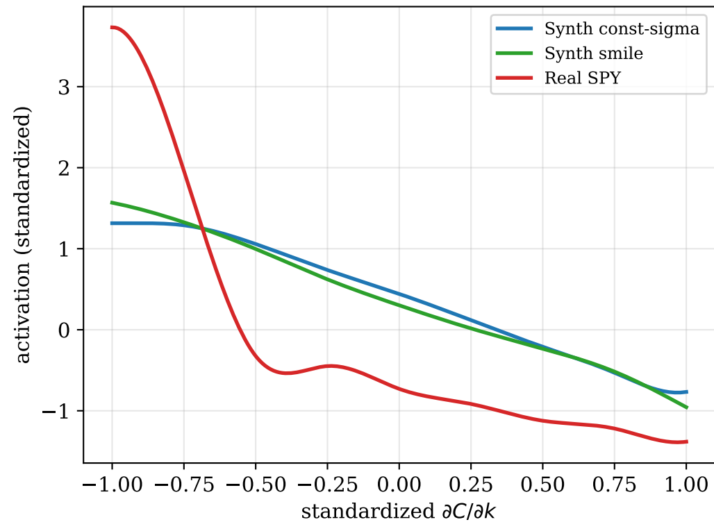
\varphi_{\text{drift}}(\partial C/\partial k)
