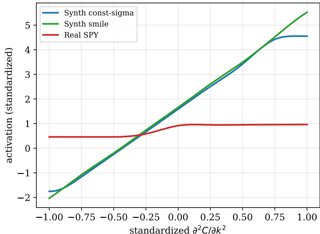
\varphi_{\text{diffusion}}(\partial^2 C/\partial k^2)
