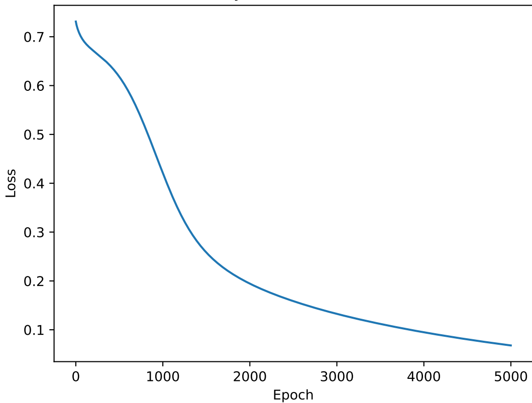
Binary Classification Loss
