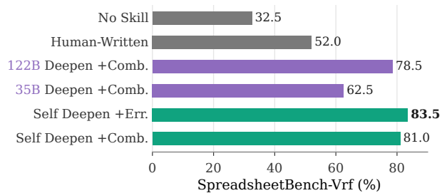
GPT-5.5 user
