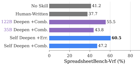
Gemma-4 user
