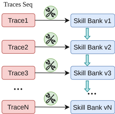
Sequential Updates of a Skill Bank
