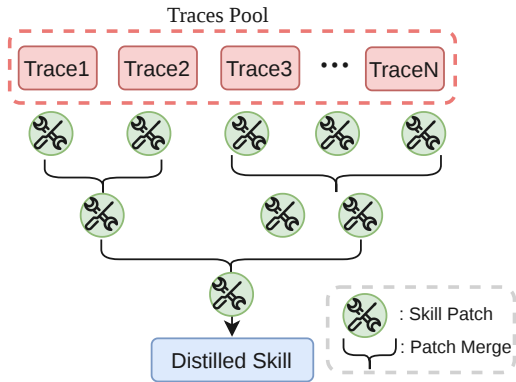
Parallel Distillation of All Lessons into a Skill
