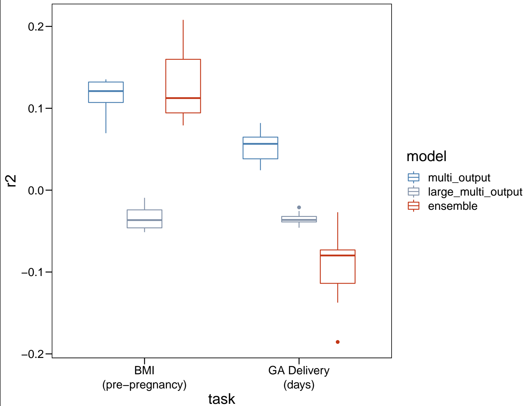
Model Performance ( R^2 )
