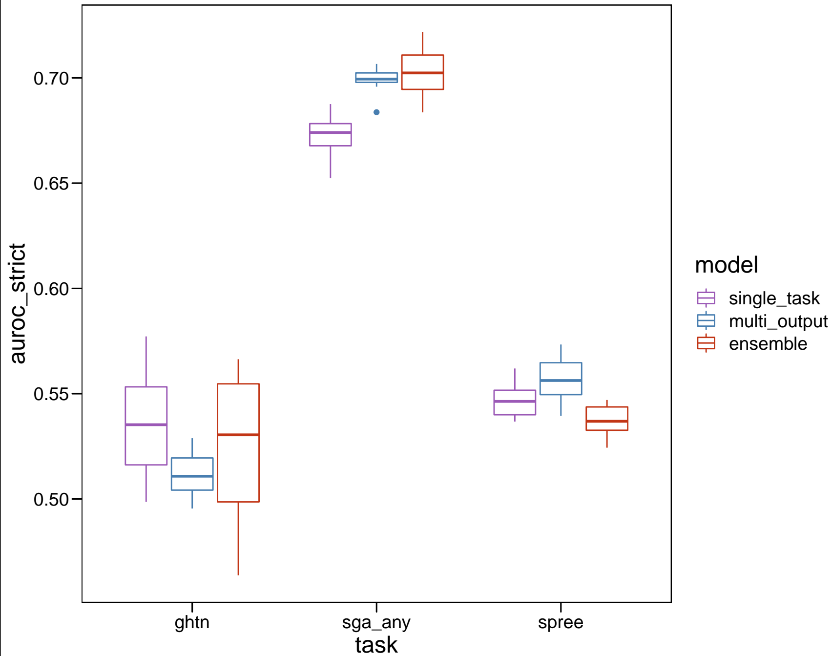
Model Performance (AUROC)
