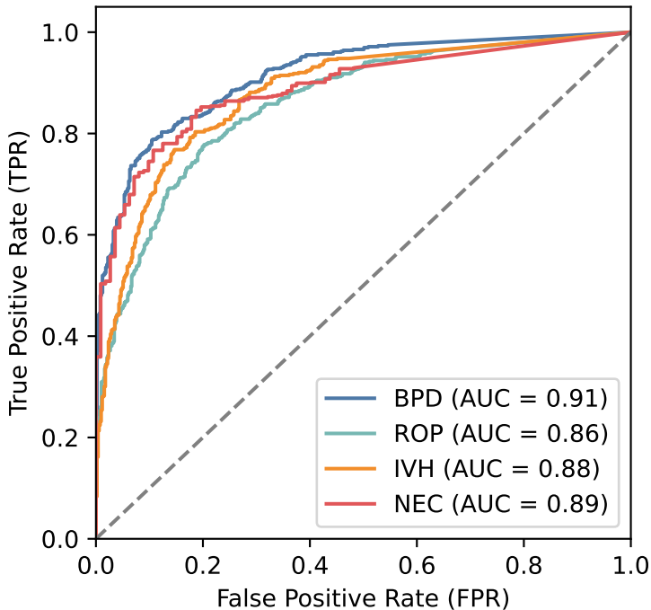
ROC Curve (Test Set)
