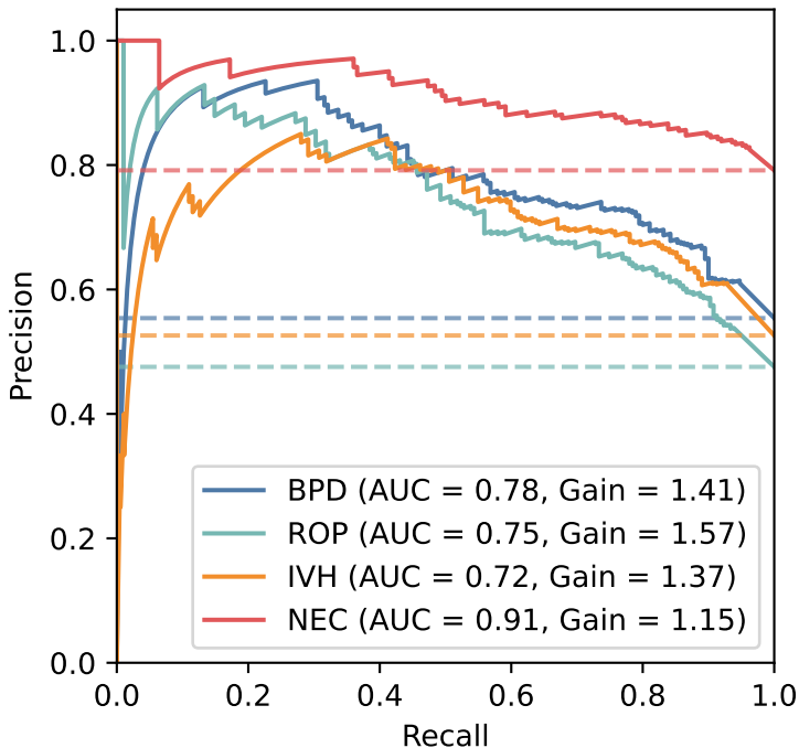
PR Curve (Validation Set)
