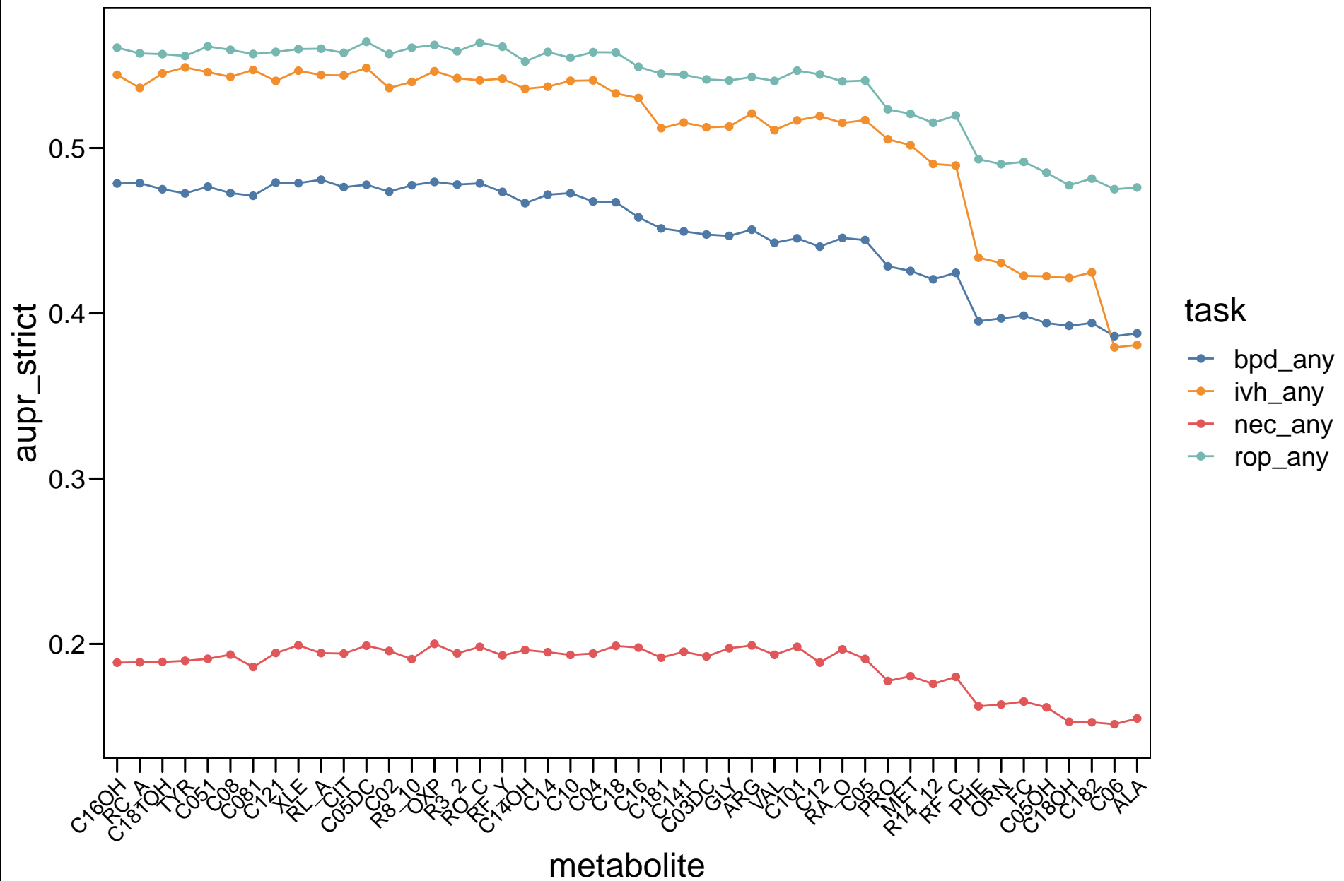
feature ranks: ivh_any , model: ensemble
