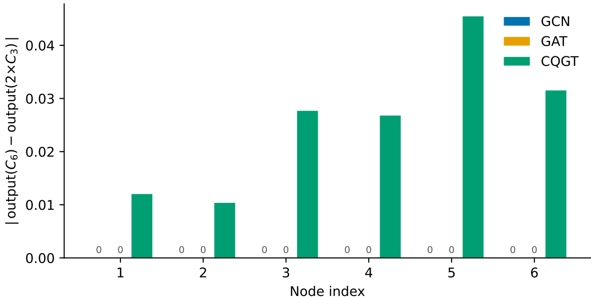
1-WL separation: C_6 vs. 2 \times C_3 , identical node features
