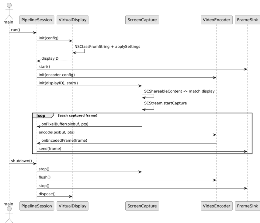
Figure 2: Actor diagram for lifetimes of the client. Showcases the loop of frame encoding and sending to the headset to FrameSink
