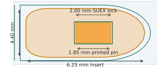
orange: STL insert projection; green: SUEX lock outline
