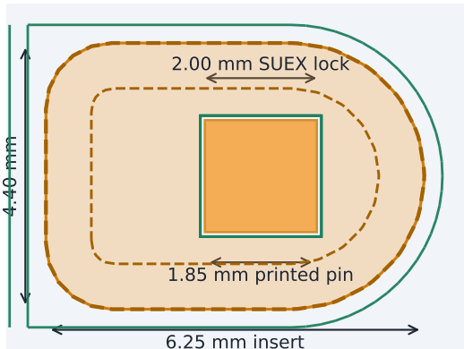
D Bonding fixture cross-section
