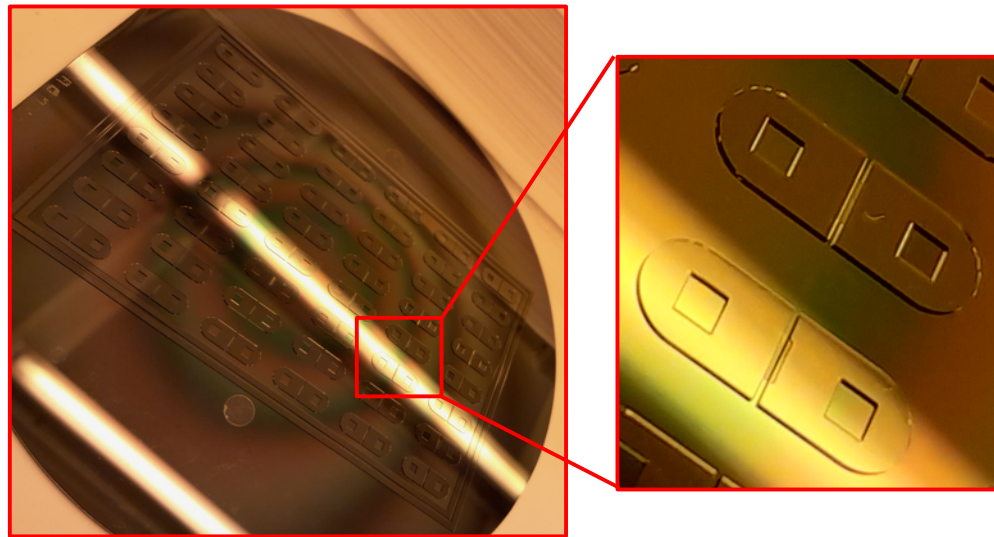
SUEX 200 with 360nm Long-Pass Filter
