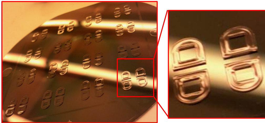
SUEX 200 without 360nm Long-Pass Filter
