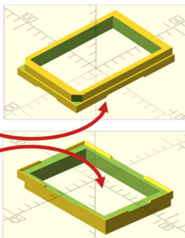
Assembly with 3D printed plates and glue
