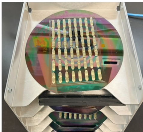
Unified mold and custom rack for parallel fabrication of devices
