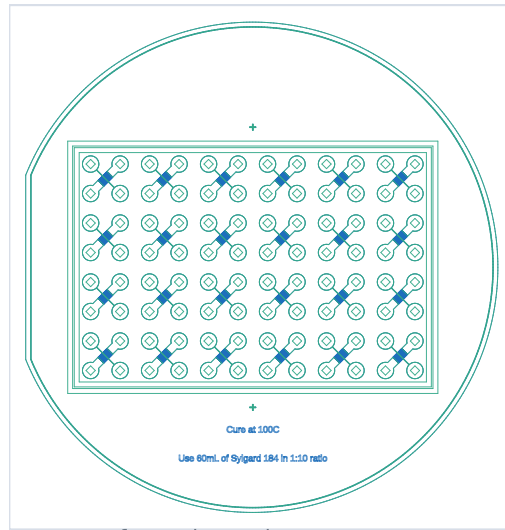
wafer-scale mask
