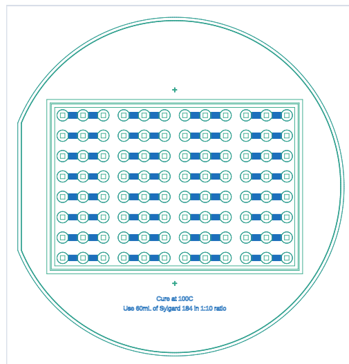
wafer-scale mask
