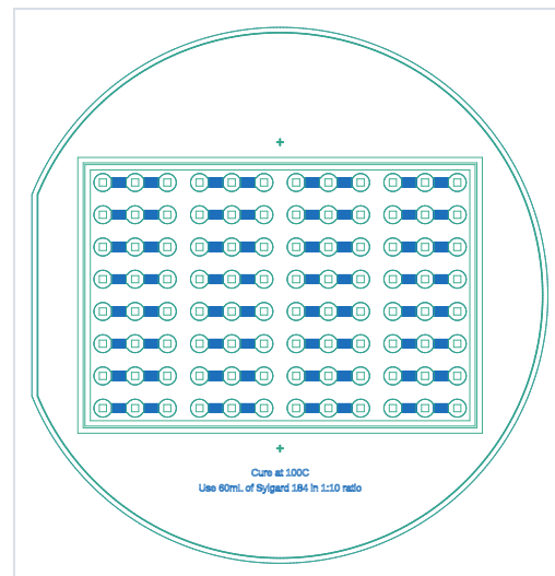
wafer-scale mask
