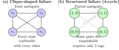
Figure 1: Two failure topologies. In (a), the observation provides no discrimination, so the confusability graph is a clique: every state is confusable with every other, and exact recovery requires a tag for each state. In (b), partial observations provide some discrimination: opposite corners are distinguishable even though adjacent states are not. The 4-cycle is 2-colorable, so exact recovery requires only 2 tags. This structural difference is invisible to the unit-rate threshold alone.
