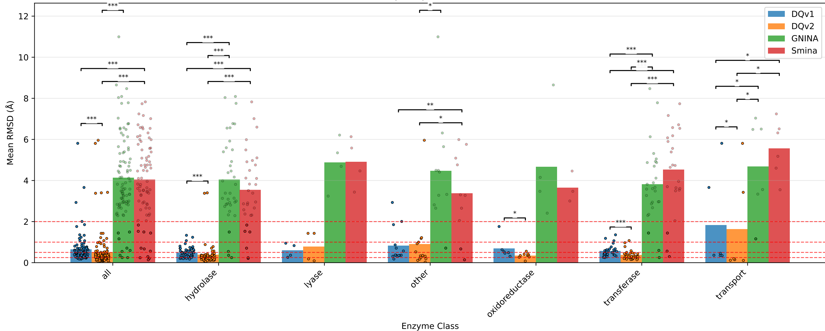
Mean RMSD by Enzyme Class and Method
