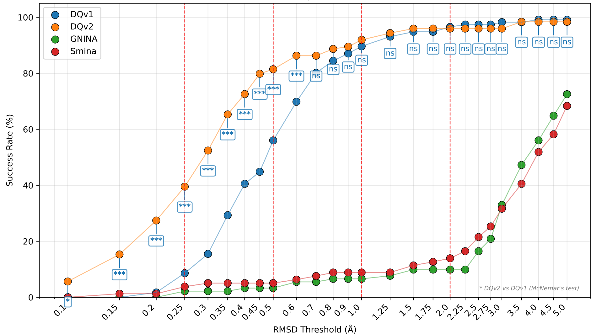
Success Rate by RMSD Threshold
