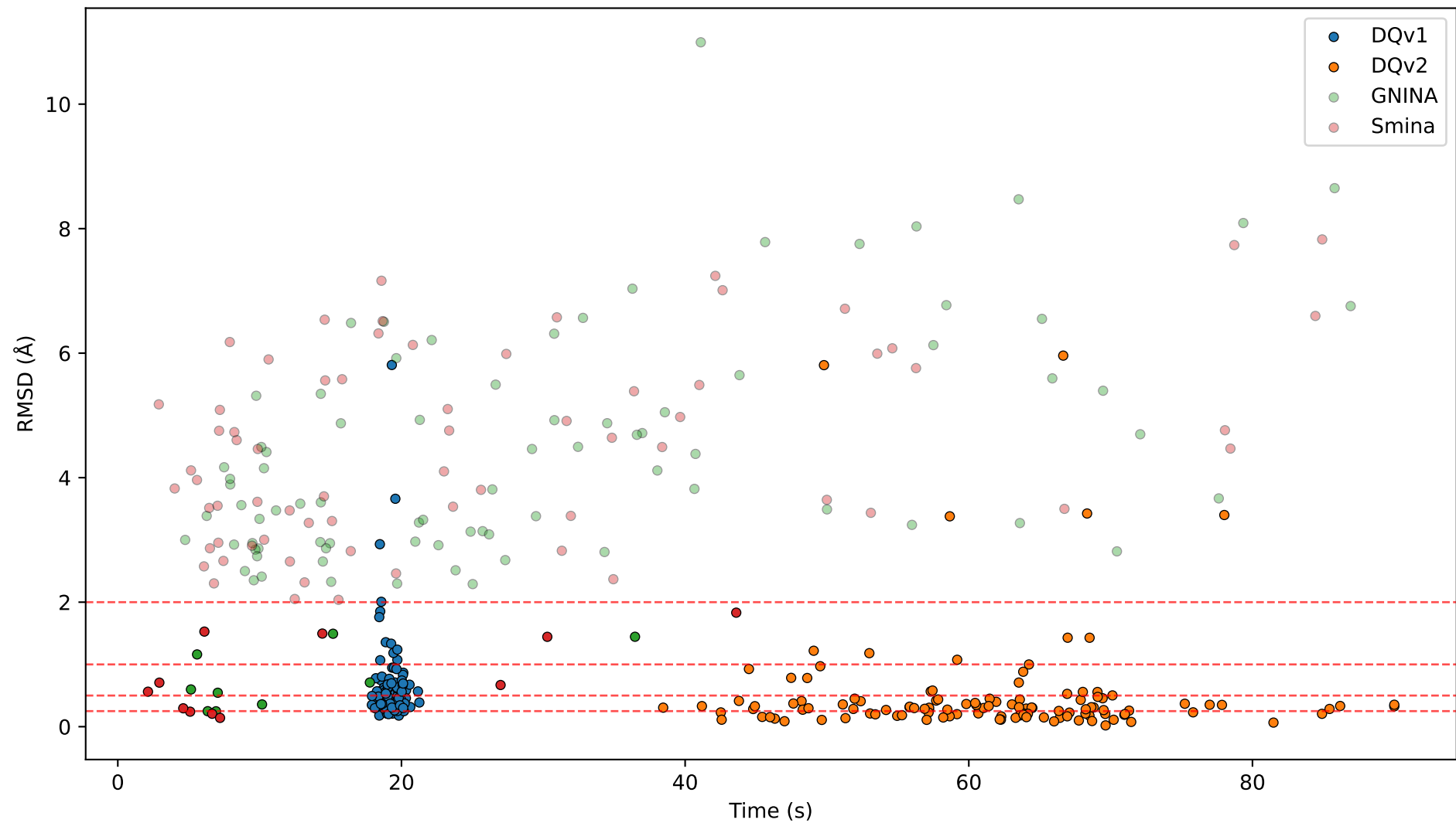
Runtime vs RMSD
