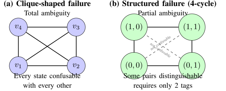
Fig. 1. Two failure topologies. In (a), the observation provides no discrimination, so the confusability graph is a clique: every state is confusable with every other, and exact recovery requires a tag for each state. In (b), partial observations provide some discrimination: opposite corners are distinguishable even though adjacent states are not. The 4-cycle is 2-colorable, so exact recovery requires only 2 tags. This structural difference is invisible to the unit-rate threshold alone.
