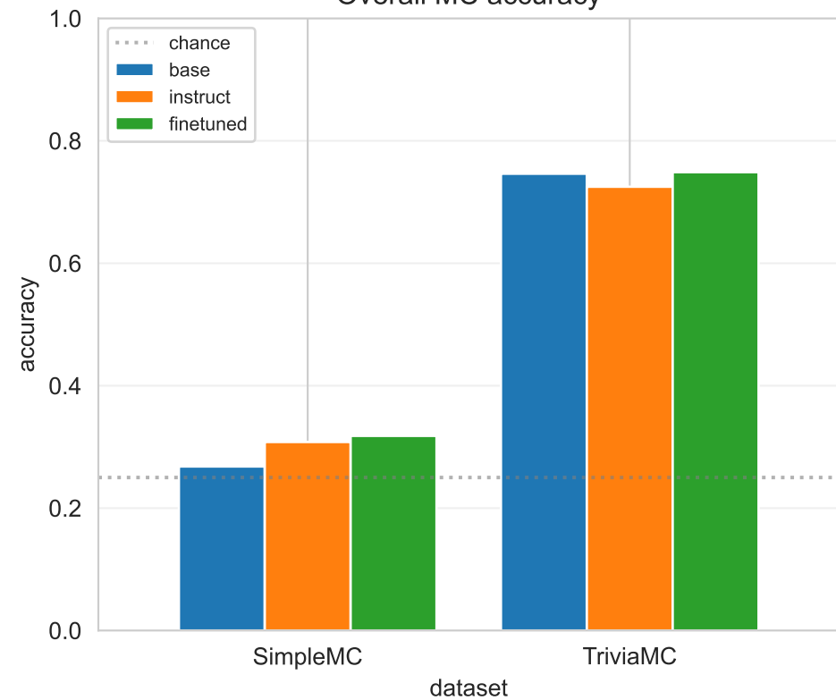
Overall MC accuracy
