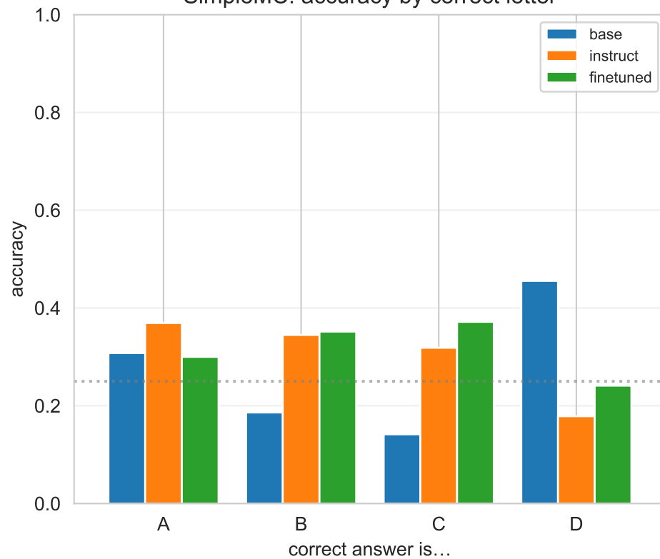
SimpleMC: accuracy by correct letter
