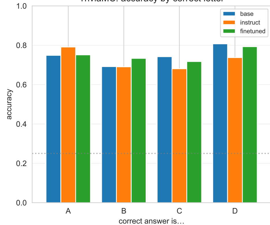
TriviaMC: accuracy by correct letter
