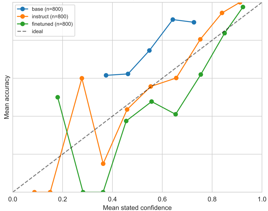
Reliability: TriviaMC
