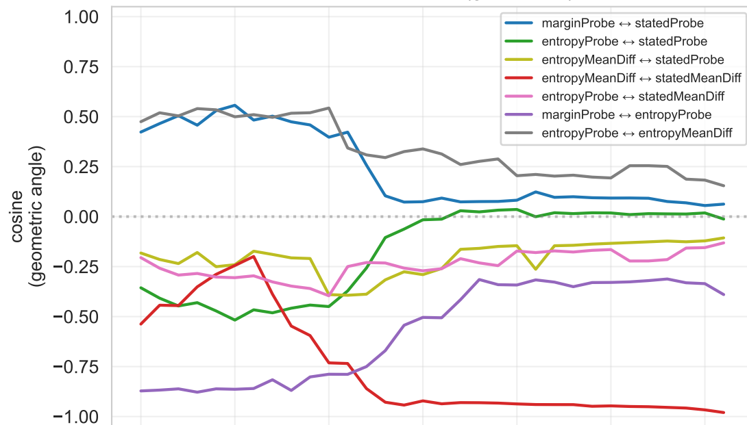
instruct — cosine (geometric)
