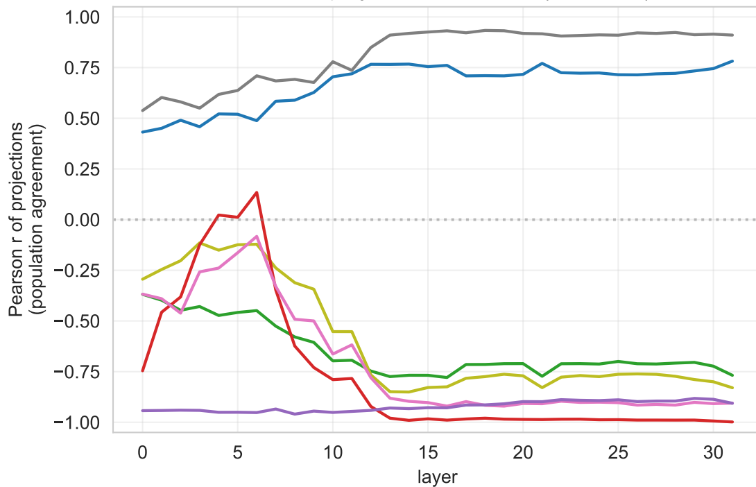
instruct — projection correlation (functional)
