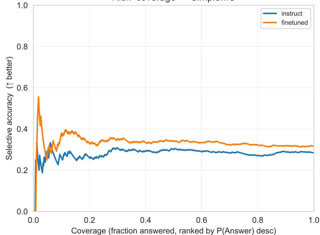
Risk-coverage — SimpleMC
